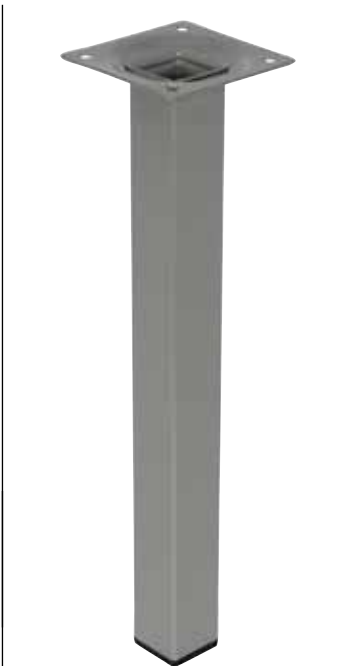
1107509 - Furniture leg square Colour: Grey Material & finish: Steel, PVC Dimension: 2,5x2,5x25 cm Loading weight: 50 kg Quantity: 4
