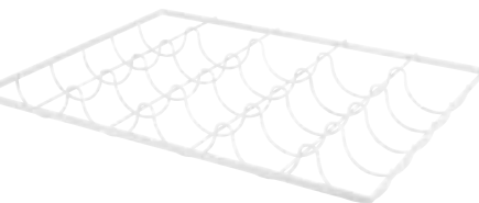
1204950 - Storage-system wine bottle rack Colour: White Material & finish: Steel, powdercoated Dimension: 56,9x46x6 cm Loading weight: 15 kg Quantity: 3
