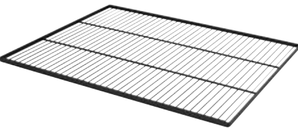
1204939 - Storage-system shelf wire Colour: Black Material & finish: Steel, powdercoated Dimension: 56,9x46x1,5 cm Loading weight: 25 kg Quantity: 4
