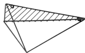
1207803 - Wall shelf triangle lines Color: Black Material & finish: Steel, powdercoated Dimensions: 26x15x12,5 cm Loading weight: 1 kg Quantity: 4
