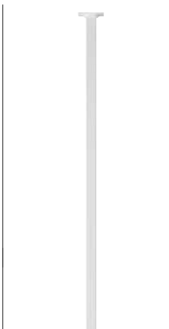
1107514 - Furniture leg square Colour: White Material & finish: Steel, PVC Dimension: 2,5x2,5x75 cm Loading weight: 50 kg Quantity: 4
