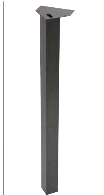
1107484 - Furniture leg square Colour: Anthracite Material & finish: Steel, PVC Dimension: 5x5x72 cm Loading weight: 100 kg Quantity: 4
