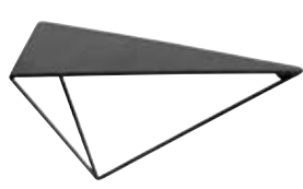
1207813 - Wall shelf triangle Color: Black Material & finish: Steel, powdercoated Dimensions: 26x15x12,5 cm Loading weight: 1 kg Quantity: 4
