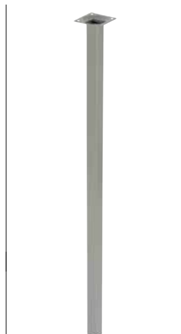
1107512 - Furniture leg square Colour: Grey Material & finish: Steel, PVC Dimension: 2,5x2,5x75 cm Loading weight: 50 kg Quantity: 4
